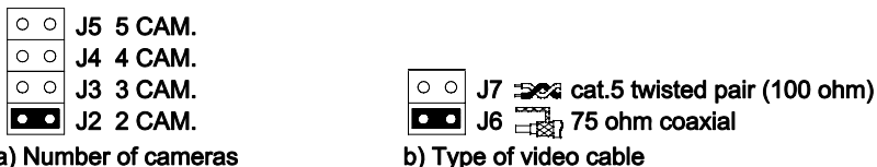
FIGURE 1. Exchanger configuration
